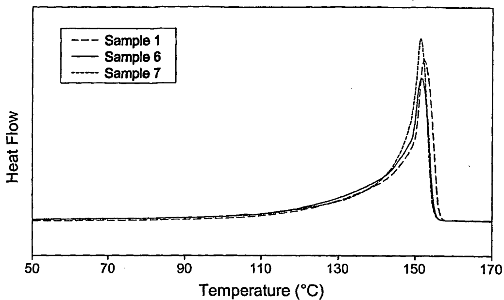
Fig. 5 DSC Melting of Plasticized Metallocene Propylene Polymers
